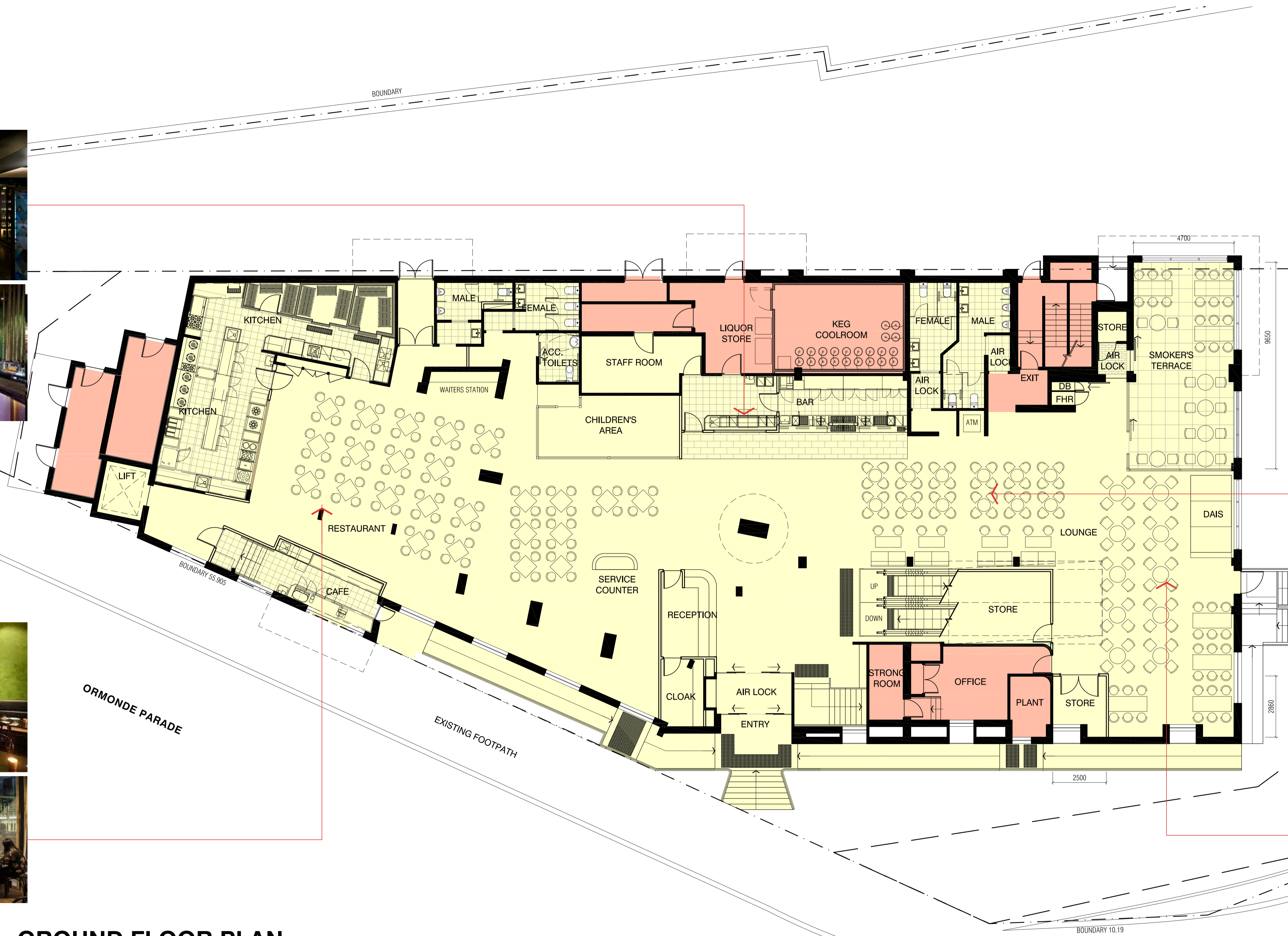
01 GROUND FLOOR PLAN SCALE 1:100 @ A1
